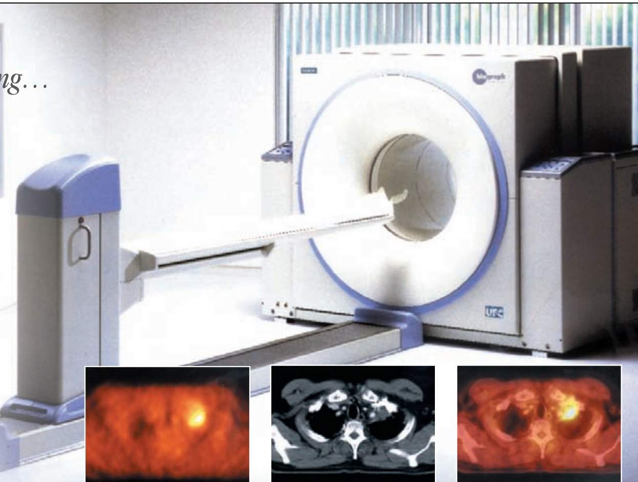
PET Image-Chest
