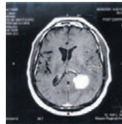
Brain Imaging
